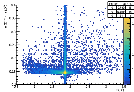
Failed non-DiF ( 0 < n_{\text{Tracks}} < 200 , 3.6 < \eta < 5.0 , 60000 < p < 100000 )
