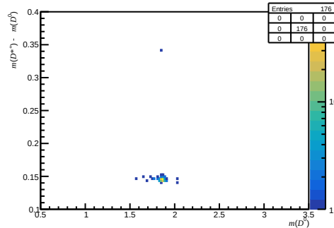
Passed non-DiF ( 0 < n_{\text{Tracks}} < 200 , 3.6 < \eta < 5.0 , 60000 < p < 100000 )
