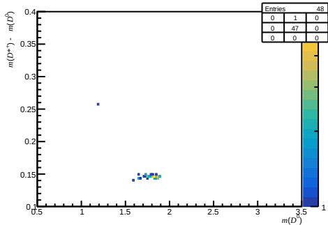
Passed DiF - after RICH1 ( 0 < n_{\text{Tracks}} < 200 , 3.6 < \eta < 5.0 , 60000 < p < 100000 )
