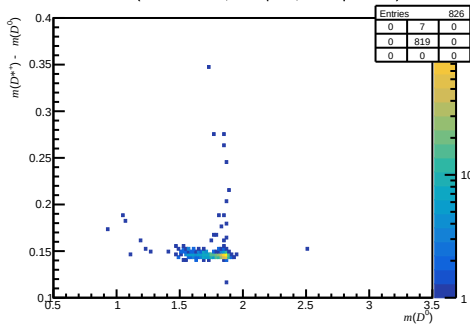
Failed DiF ( 0 < n_{\text{Tracks}} < 200 , 3.6 < \eta < 5.0 , 60000 < p < 100000 )
