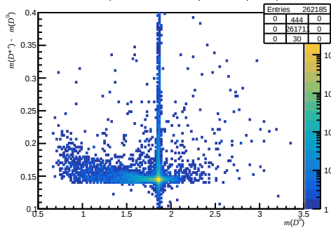
Failed non-DiF (200 < nTracks < 600, 1.7 < \eta < 3.6, 27000 < p < 60000)
