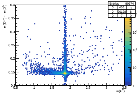
Failed non-DiF (200 < nTracks < 600, 3.6 < \eta < 5.0, 60000 < p < 100000)
