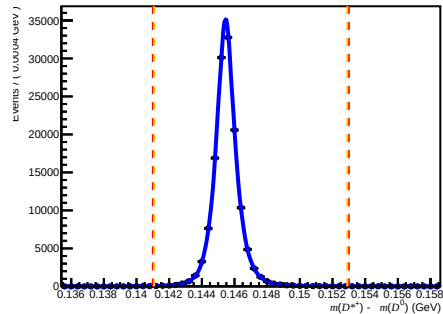
Failed DIF ( 0 < nTracks < 200 , 1.7 < \eta < 3.6 , 6000 < p < 10000 )
