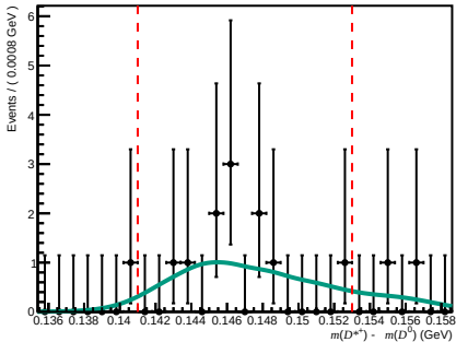
Passed ( 0 < n\text{Tracks} < 200 , 3.6 < \eta < 5.0 , 10000 < p < 15600 )
