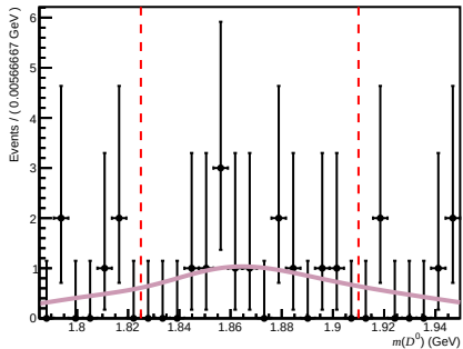
Failed ( 0 < n\text{Tracks} < 200 , 3.6 < \eta < 5.0 , 27000 < p < 60000 )
