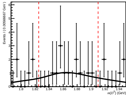
Total ( 200 < nTracks < 600 , 3.6 < \eta < 5.0 , 27000 < p < 60000 )
