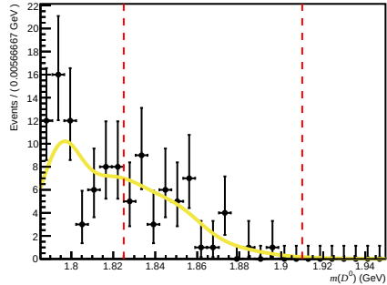
Failed ( 200 < nTracks < 600 , 3.6 < \eta < 5.0 , 60000 < p < 100000 )
