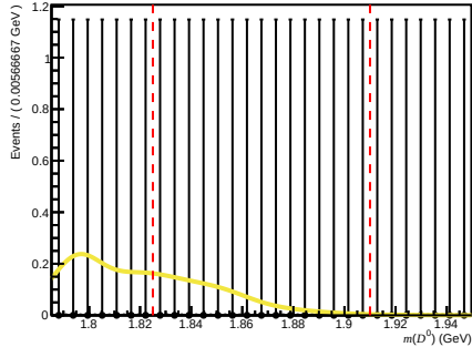
Passed ( 200 < nTracks < 600 , 3.6 < \eta < 5.0 , 60000 < p < 100000 )
