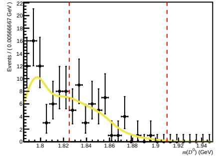
Total ( 200 < nTracks < 600 , 3.6 < \eta < 5.0 , 60000 < p < 100000 )
