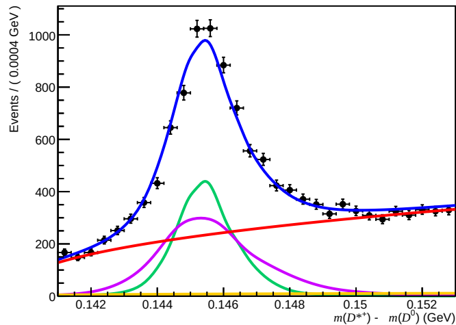
Failed ( 0 < n_{\text{Tracks}} < 200 , 1.7 < \eta < 3.6 , 3000 < p < 6000 )
