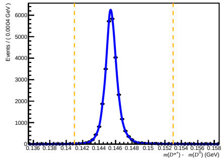
Passed DiF (after RICH1) ( 0 < nTracks < 200 , 1.7 < \eta < 3.6 , 27000 < p < 60000 )
