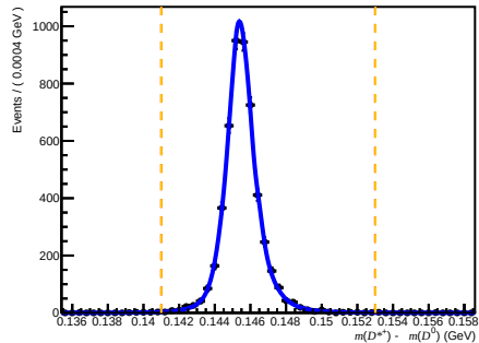
Failed DiF ( 0 < nTracks < 200 , 1.7 < \eta < 3.6 , 27000 < p < 60000 )
