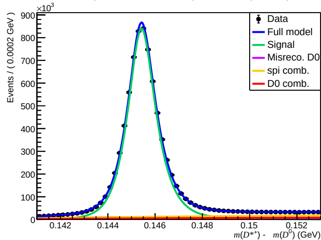
Failed ( 0 < n_{\text{Tracks}} < 200 , 1.7 < \eta < 3.6 , 27000 < p < 60000 )
