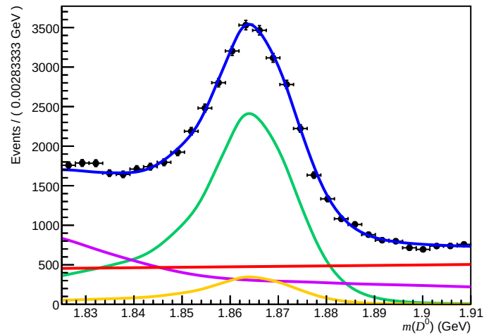
Failed ( 0 < n_{\text{Tracks}} < 200 , 1.7 < \eta < 3.6 , 27000 < p < 60000 )
