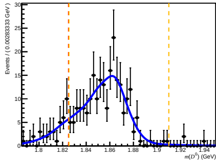
Failed DIF ( 0 < n_{\text{Tracks}} < 200 , 1.7 < \eta < 3.6 , 60000 < p < 100000 )
