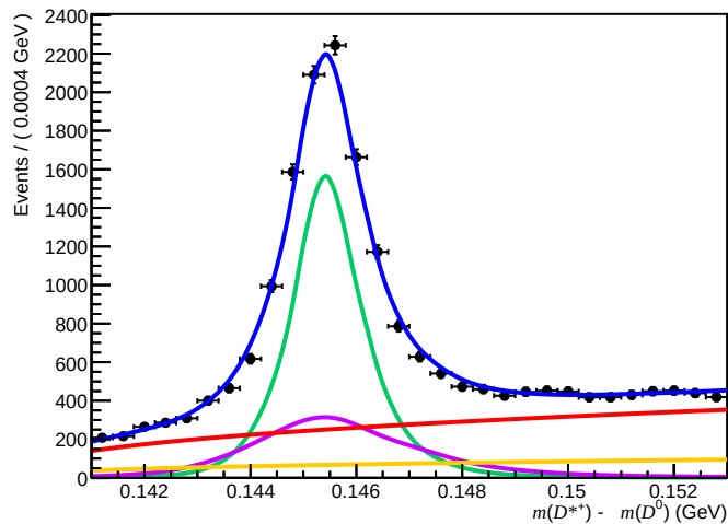
Passed (200 < nTracks < 600, 1.7 < \eta < 3.6, 6000 < p < 10000)
