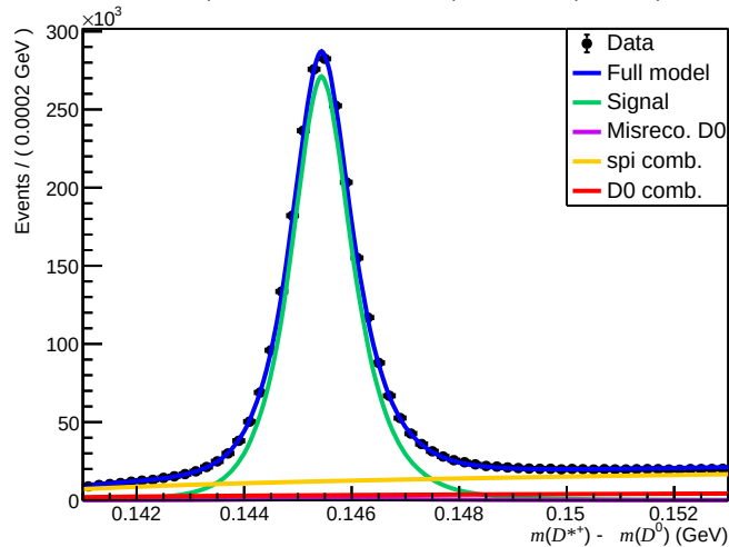
Failed (200 < nTracks < 600, 1.7 < \eta < 3.6, 6000 < p < 10000)
