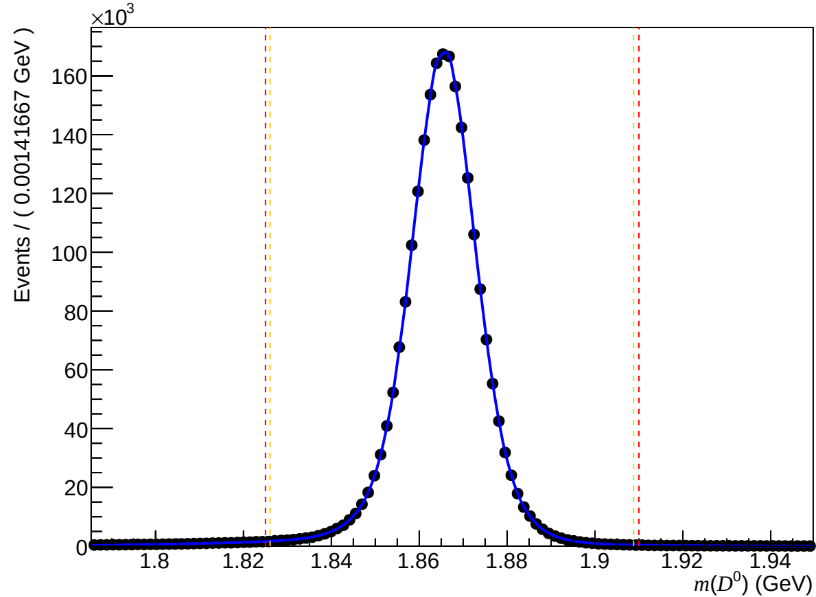
Failed non-DiF ( 200 < nTracks < 600 , 1.7 < \eta < 3.6 , 15600 < p < 27000 )
