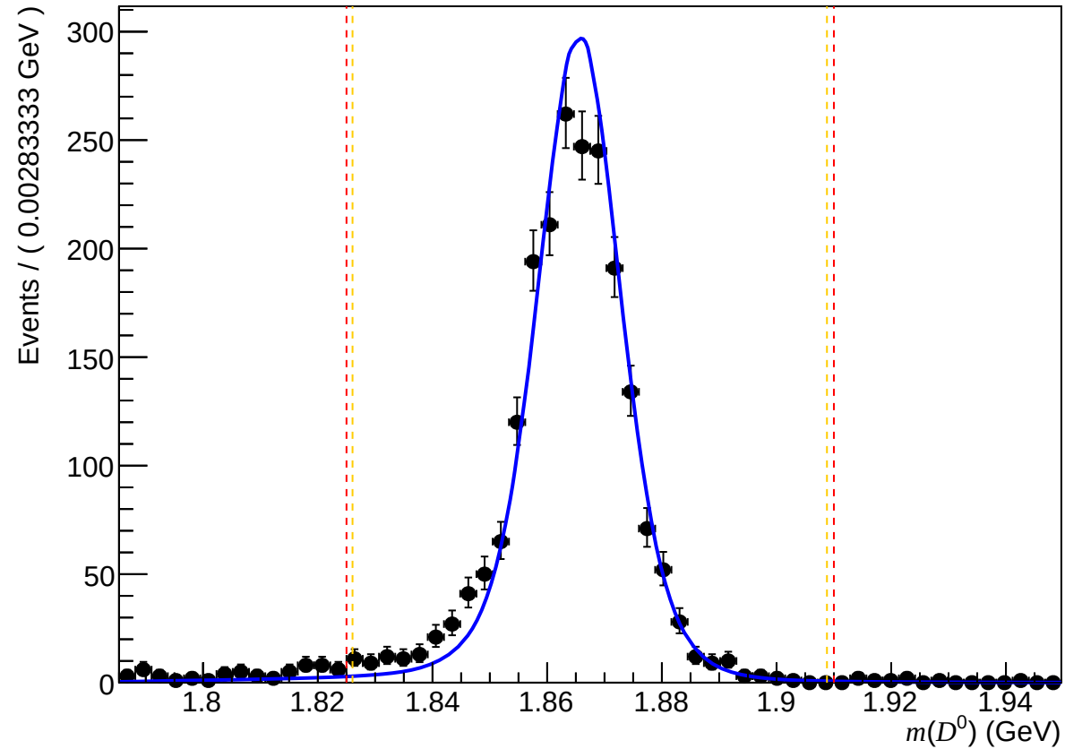
Passed non-DiF ( 200 < nTracks < 600 , 1.7 < \eta < 3.6 , 15600 < p < 27000 )
