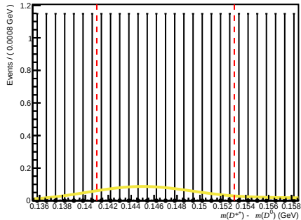
Passed ( 200 < nTracks < 600 , 1.7 < \eta < 3.6 , 60000 < p < 100000 )
