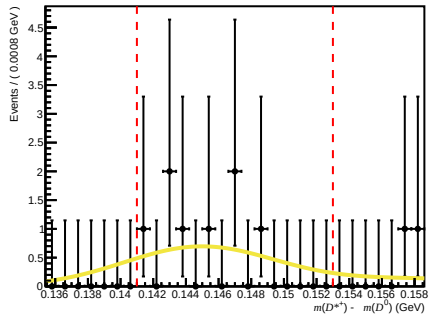
Failed ( 200 < nTracks < 600 , 1.7 < \eta < 3.6 , 60000 < p < 100000 )
