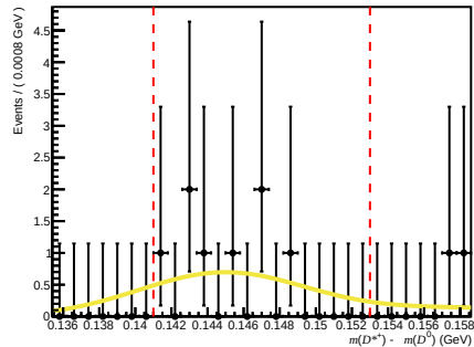
Total ( 200 < nTracks < 600 , 1.7 < \eta < 3.6 , 60000 < p < 100000 )
