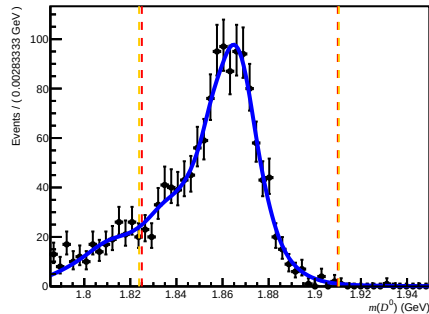
Failed DiF ( 200 < nTracks < 600 , 3.6 < \eta < 5.0 , 27000 < p < 60000 )
