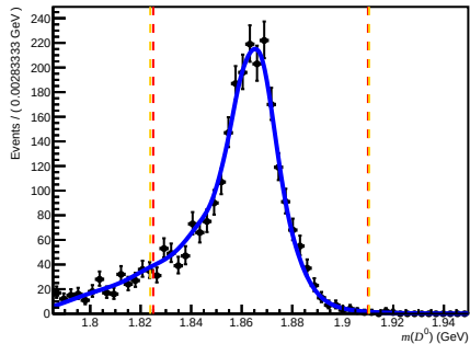
Passed DiF (after RICH1) ( 200 < nTracks < 600 , 3.6 < \eta < 5.0 , 27000 < p < 60000 )
