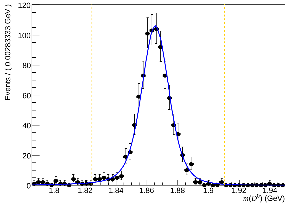
Passed non-DiF ( 200 < nTracks < 600 , 3.6 < \eta < 5.0 , 27000 < p < 60000 )
