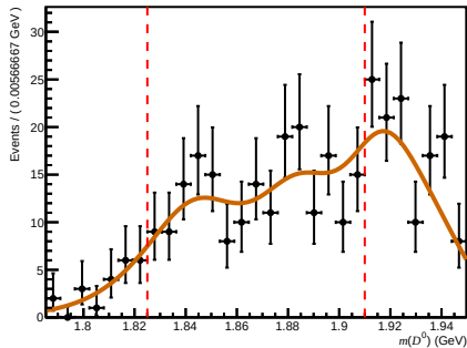
Total ( 0 < n_{\text{Tracks}} < 200 , 3.6 < \eta < 5.0 , 3000 < p < 6000 )
