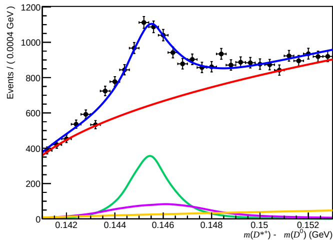
Failed ( 0 < n\text{Tracks} < 200 , 3.6 < \eta < 5.0 , 15600 < p < 27000 )
