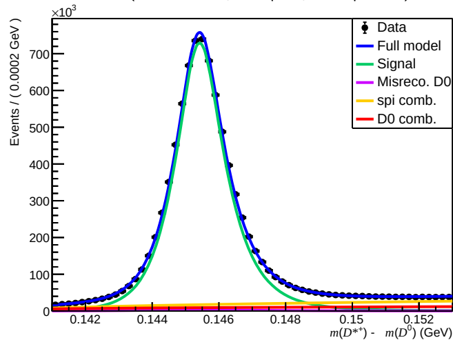
Failed ( 0 < n\text{Tracks} < 200 , 3.6 < \eta < 5.0 , 27000 < p < 60000 )
