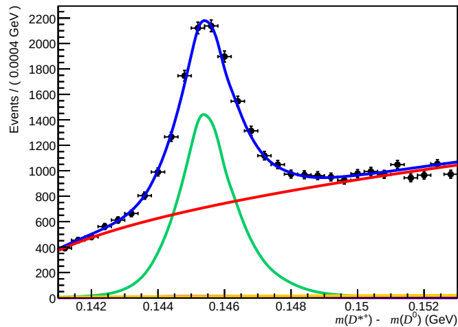
Failed ( 0 < n\text{Tracks} < 200 , 3.6 < \eta < 5.0 , 27000 < p < 60000 )
