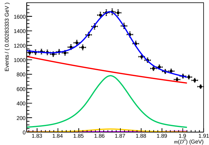
Failed ( 0 < n\text{Tracks} < 200 , 3.6 < \eta < 5.0 , 27000 < p < 60000 )
