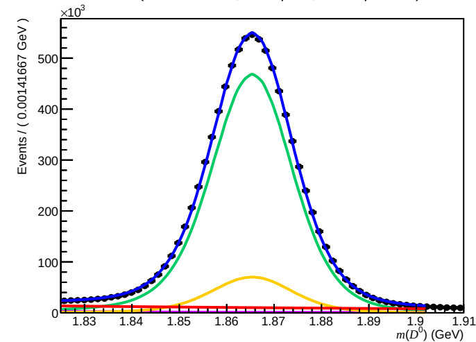
Failed ( 0 < n\text{Tracks} < 200 , 3.6 < \eta < 5.0 , 27000 < p < 60000 )
