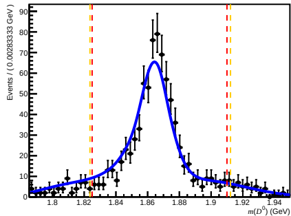
Passed DiF (after RICH1) ( 200 < nTracks < 600 , 1.7 < \eta < 3.6 , 15600 < p < 27000 )
