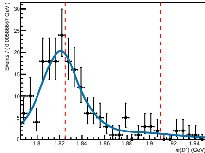
Total ( 200 < n_{\text{Tracks}} < 600 , 3.6 < \eta < 5.0 , 6000 < p < 10000 )
