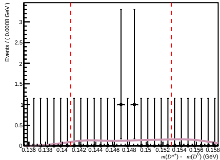
Passed ( 200 < n\text{Tracks} < 600 , 3.6 < \eta < 5.0 , 6000 < p < 10000 )
