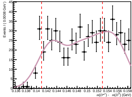
Total ( 200 < n\text{Tracks} < 600 , 3.6 < \eta < 5.0 , 6000 < p < 10000 )
