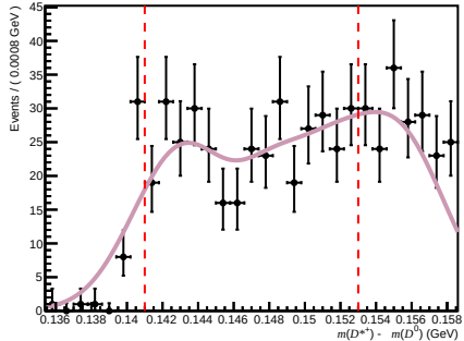
Failed ( 200 < n\text{Tracks} < 600 , 3.6 < \eta < 5.0 , 6000 < p < 10000 )
