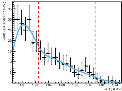
Failed ( 200 < nTracks < 600 , 3.6 < \eta < 5.0 , 60000 < p < 100000 )
