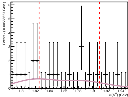
Total ( 0 < n_{\text{Tracks}} < 200 , 1.7 < \eta < 3.6 , 3000 < p < 6000 )
