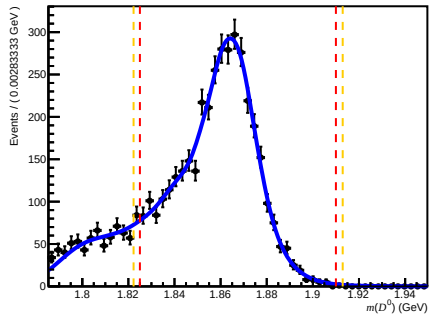
Passed DiF (after RICH1) ( 0 < n_{\text{Tracks}} < 200 , 3.6 < \eta < 5.0 , 10000 < p < 15600 )
