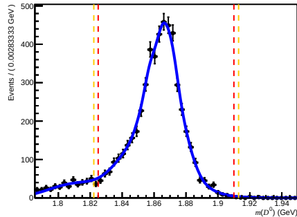
Failed DiF ( 0 < n_{\text{Tracks}} < 200 , 3.6 < \eta < 5.0 , 10000 < p < 15600 )
