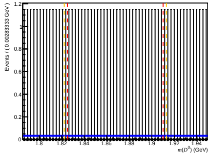
Passed DiF (before RICH1) ( 0 < n_{\text{Tracks}} < 200 , 3.6 < \eta < 5.0 , 10000 < p < 15600 )
