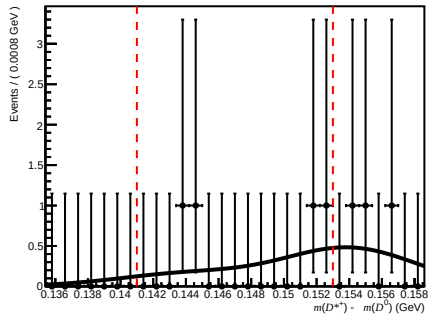
Failed ( 0 < nTracks < 200 , 3.6 < \eta < 5.0 , 10000 < p < 15600 )
