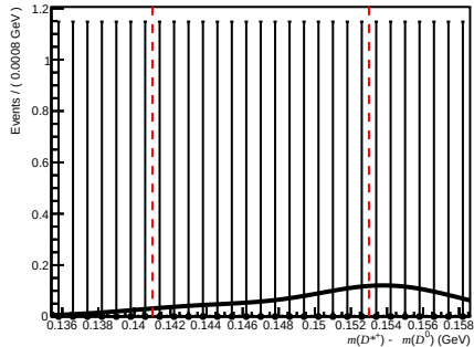
Passed ( 0 < nTracks < 200 , 3.6 < \eta < 5.0 , 10000 < p < 15600 )
