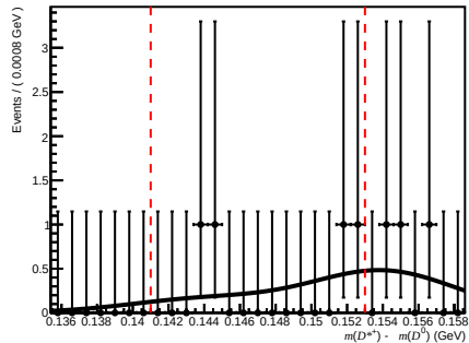
Total ( 0 < nTracks < 200 , 3.6 < \eta < 5.0 , 10000 < p < 15600 )
