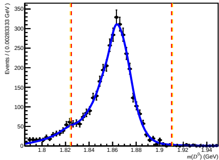
Passed DIF (after RICH1) ( 0 < n_{\text{Tracks}} < 200 , 3.6 < \eta < 5.0 , 60000 < p < 100000 )
