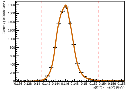
Failed ( 200 < nTracks < 600 , 1.7 < \eta < 3.6 , 6000 < p < 10000 )
