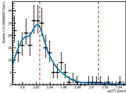
Passed ( 200 < n_{\text{Tracks}} < 600 , 1.7 < \eta < 3.6 , 60000 < p < 100000 )
