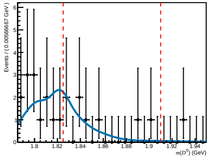
Failed ( 200 < n_{\text{Tracks}} < 600 , 1.7 < \eta < 3.6 , 60000 < p < 100000 )
