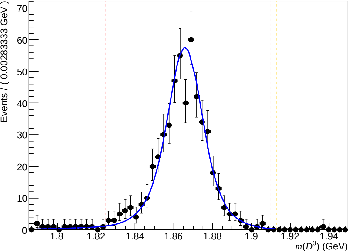
Passed non-DiF ( 200 < nTracks < 600 , 3.6 < \eta < 5.0 , 15600 < p < 27000 )
