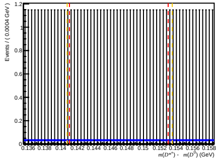
Passed DIF (before RICH1) ( 0 < nTracks < 200 , 3.6 < \eta < 5.0 , 6000 < p < 10000 )
