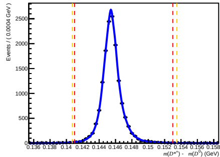
Failed DIF ( 0 < nTracks < 200 , 3.6 < \eta < 5.0 , 6000 < p < 10000 )
