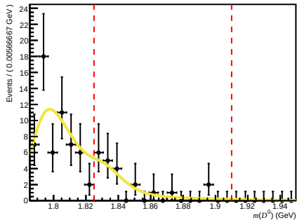
Failed ( 0 < nTracks < 200 , 3.6 < \eta < 5.0 , 15600 < p < 27000 )
