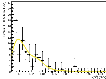
Total ( 0 < nTracks < 200 , 3.6 < \eta < 5.0 , 15600 < p < 27000 )
