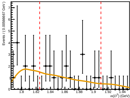
Passed ( 0 < n\text{Tracks} < 200 , 3.6 < \eta < 5.0 , 15600 < p < 27000 )
