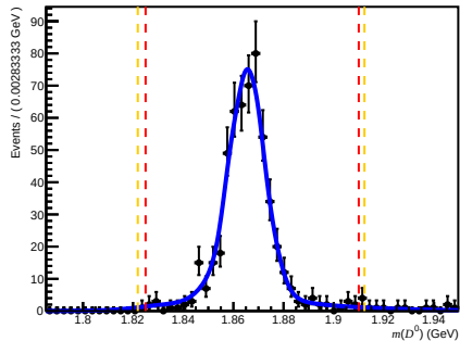
Passed DiF (after RICH1) ( 200 < n\text{Tracks} < 600 , 1.7 < \eta < 3.6 , 3000 < p < 6000 )
