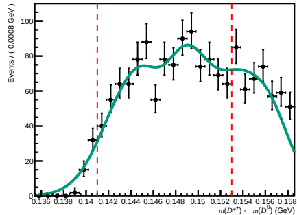
Total ( 200 < nTracks < 600 , 1.7 < \eta < 3.6 , 3000 < p < 6000 )
