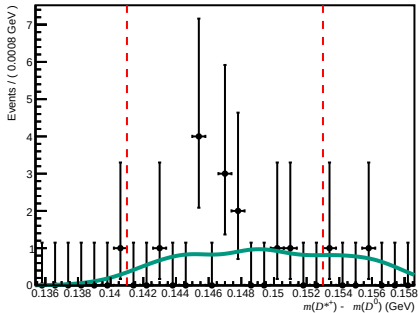
Passed ( 200 < nTracks < 600 , 1.7 < \eta < 3.6 , 3000 < p < 6000 )
