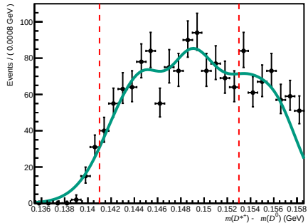
Failed ( 200 < nTracks < 600 , 1.7 < \eta < 3.6 , 3000 < p < 6000 )
