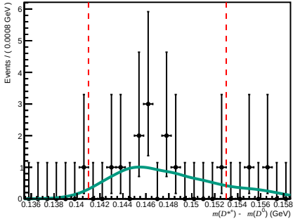
Passed ( 200 < nTracks < 600 , 1.7 < \eta < 3.6 , 10000 < p < 15600 )
