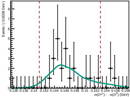
Passed ( 200 < n\text{Tracks} < 600 , 1.7 < \eta < 3.6 , 15600 < p < 27000 )
