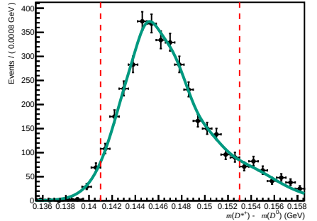
Total ( 200 < n\text{Tracks} < 600 , 1.7 < \eta < 3.6 , 15600 < p < 27000 )
