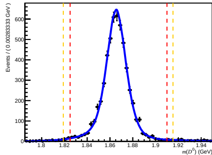
Failed DiF ( 200 < n_{\text{Tracks}} < 600 , 3.6 < \eta < 5.0 , 10000 < p < 15600 )
