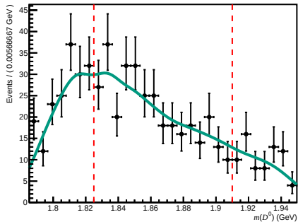
Failed ( 0 < nTracks < 200 , 1.7 < \eta < 3.6 , 15600 < p < 27000 )
