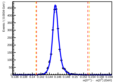
Passed DIF (after RICH1) ( 0 < nTracks < 200 , 1.7 < \eta < 3.6 , 60000 < p < 100000 )
