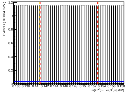
Passed DIF (before RICH1) ( 0 < nTracks < 200 , 1.7 < \eta < 3.6 , 60000 < p < 100000 )
