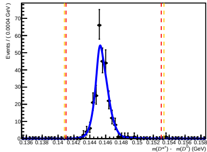
Failed DIF ( 0 < nTracks < 200 , 1.7 < \eta < 3.6 , 60000 < p < 100000 )
