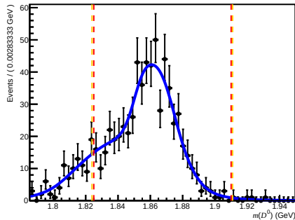
Failed DIF ( 0 < nTracks < 200 , 3.6 < \eta < 5.0 , 60000 < p < 100000 )
