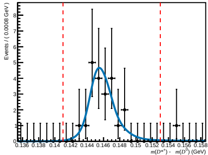
Failed ( 0 < n\text{Tracks} < 200 , 3.6 < \eta < 5.0 , 60000 < p < 100000 )
