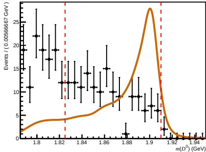
Passed ( 200 < n\text{Tracks} < 600 , 1.7 < \eta < 3.6 , 3000 < p < 6000 )
