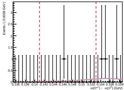
Failed ( 200 < n\text{Tracks} < 600 , 1.7 < \eta < 3.6 , 3000 < p < 6000 )
