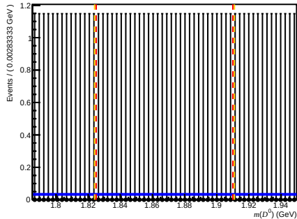
Passed DIF (before RICH1) ( 200 < n_{\text{Tracks}} < 600 , 1.7 < \eta < 3.6 , 6000 < p < 10000 )
