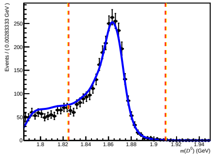
Passed DIF (after RICH1) ( 200 < n_{\text{Tracks}} < 600 , 1.7 < \eta < 3.6 , 6000 < p < 10000 )
