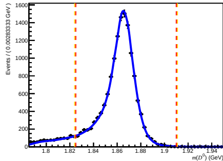
Failed DIF ( 200 < n_{\text{Tracks}} < 600 , 1.7 < \eta < 3.6 , 6000 < p < 10000 )
