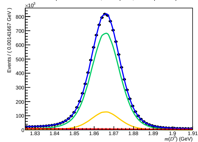
Failed ( 200 < n\text{Tracks} < 600 , 1.7 < \eta < 3.6 , 15600 < p < 27000 )
