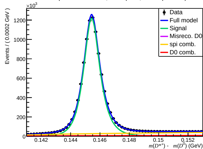
Failed ( 200 < n\text{Tracks} < 600 , 1.7 < \eta < 3.6 , 15600 < p < 27000 )
