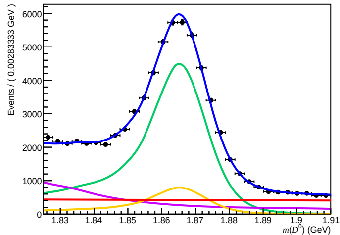
Failed ( 200 < n\text{Tracks} < 600 , 1.7 < \eta < 3.6 , 15600 < p < 27000 )
