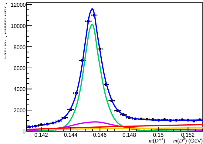
Failed ( 200 < n\text{Tracks} < 600 , 1.7 < \eta < 3.6 , 15600 < p < 27000 )
