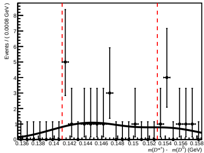
Failed ( 0 < nTracks < 200 , 1.7 < \eta < 3.6 , 27000 < p < 60000 )
