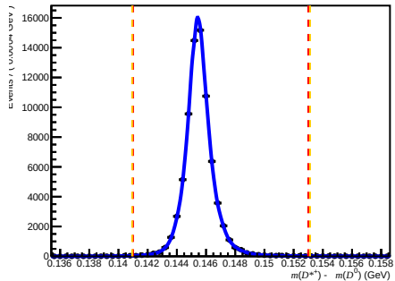
Passed DiF (after RICH1) ( 0 < n_{\text{Tracks}} < 200 , 1.7 < \eta < 3.6 , 27000 < p < 60000 )
