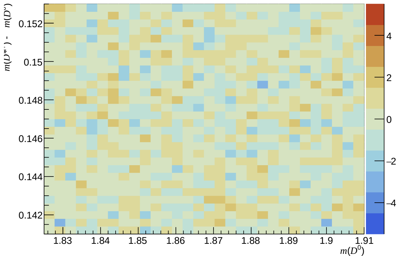
Passed ( 200 < n\text{Tracks} < 600 , 3.6 < \eta < 5.0 , 3000 < p < 6000 )
