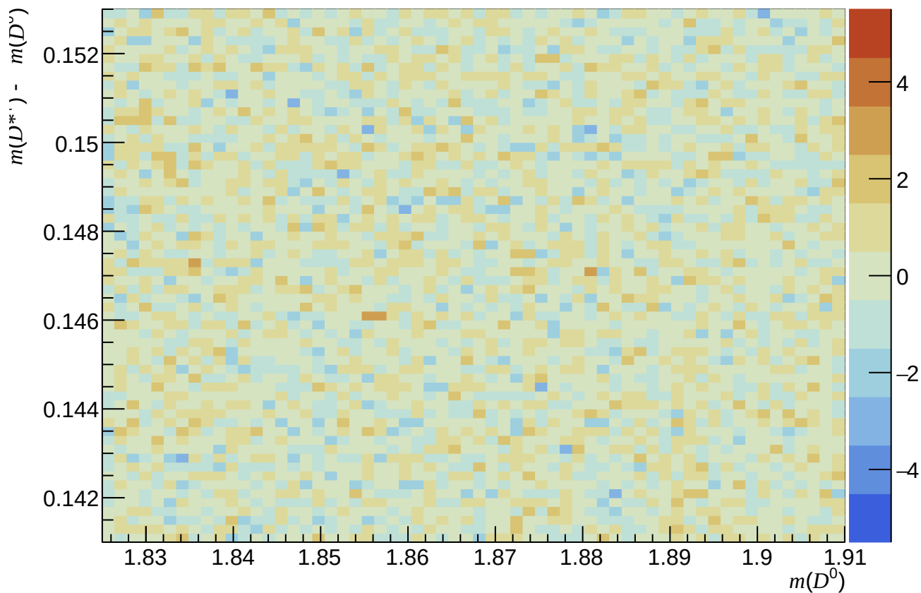
Failed ( 200 < n\text{Tracks} < 600 , 3.6 < \eta < 5.0 , 3000 < p < 6000 )
